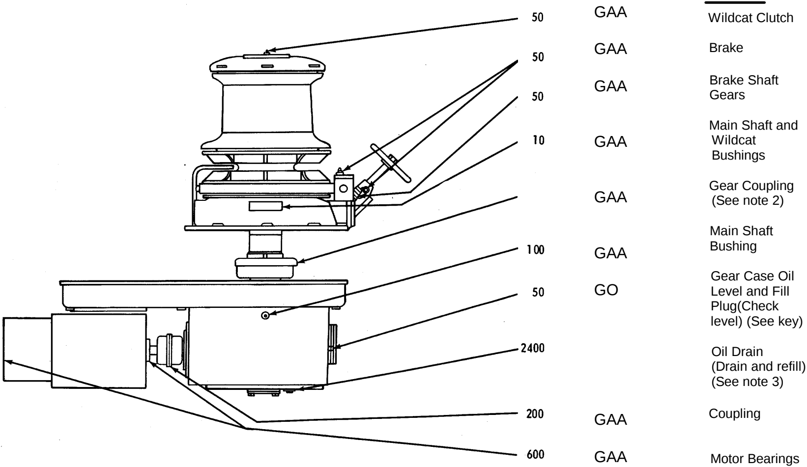
CAPSTAN-WINDLASS, MODEL VEV-16
