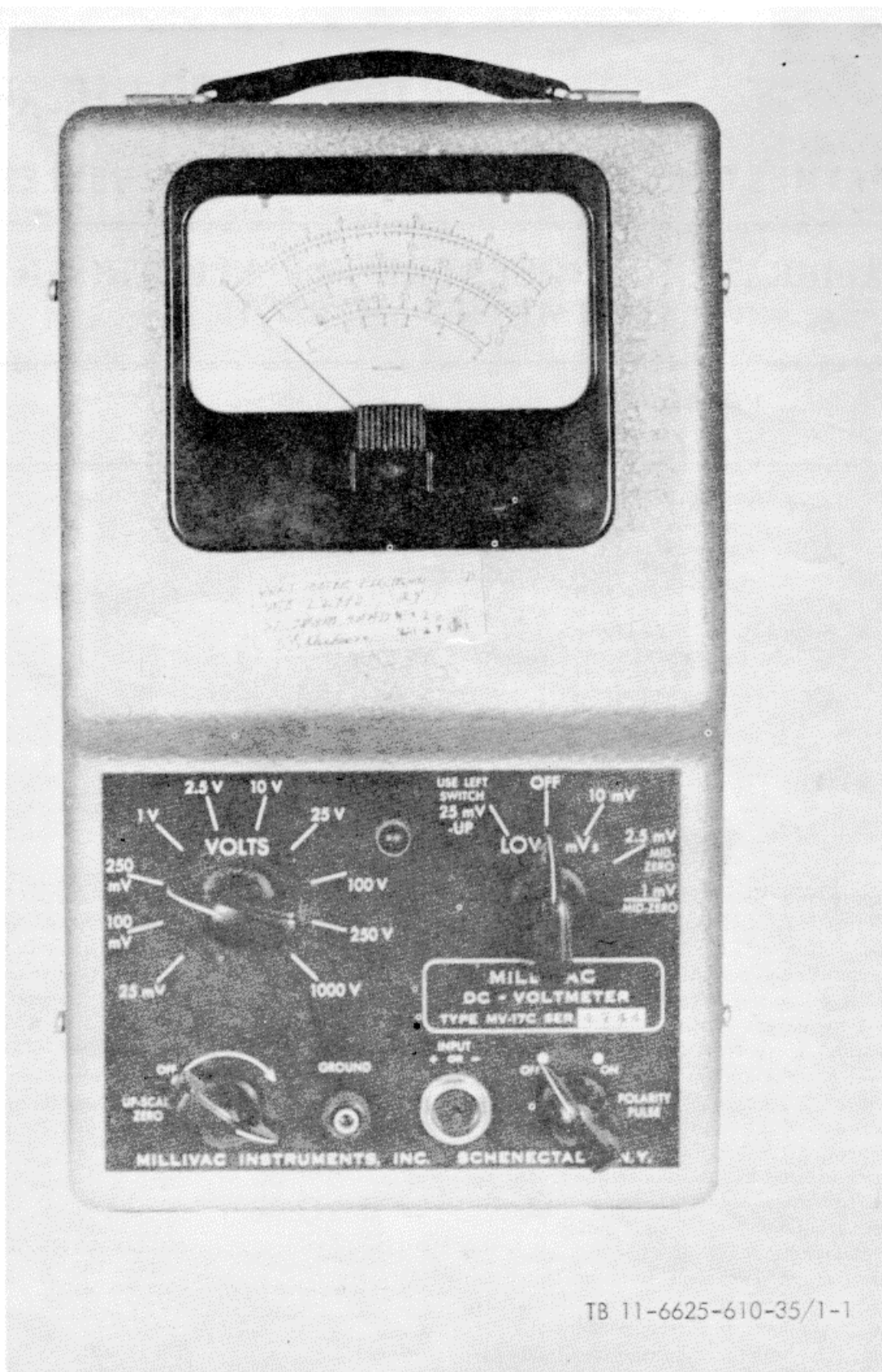
Figure 1. Electronic Voltmeter ME-227/U - front panel view.
