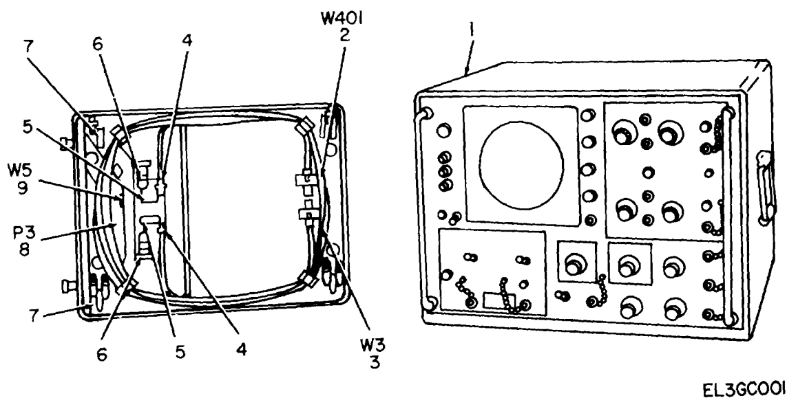
Figure 1. Oscilloscope AN/USM-140A.
