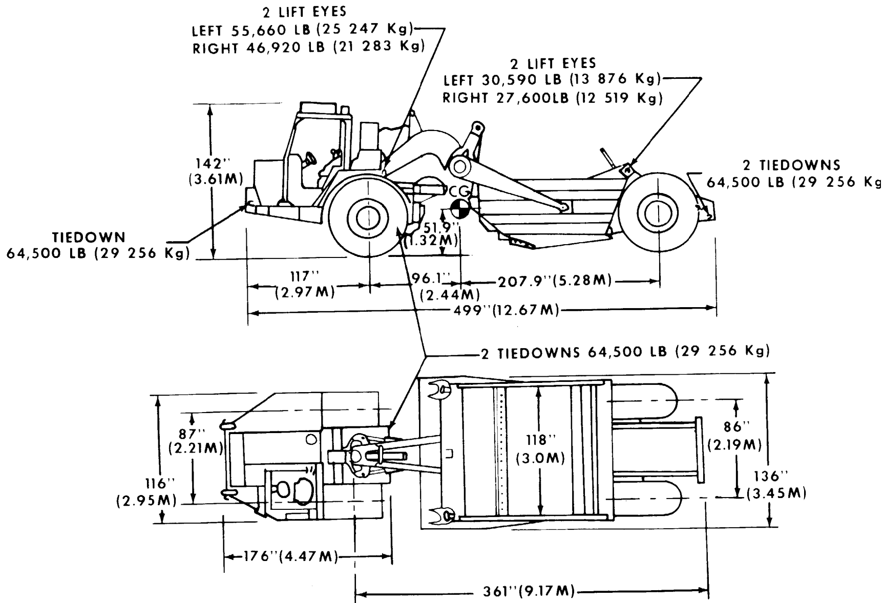
Figure 2-2. Side and top views of tractor-scraper, wheeled, M621B.
