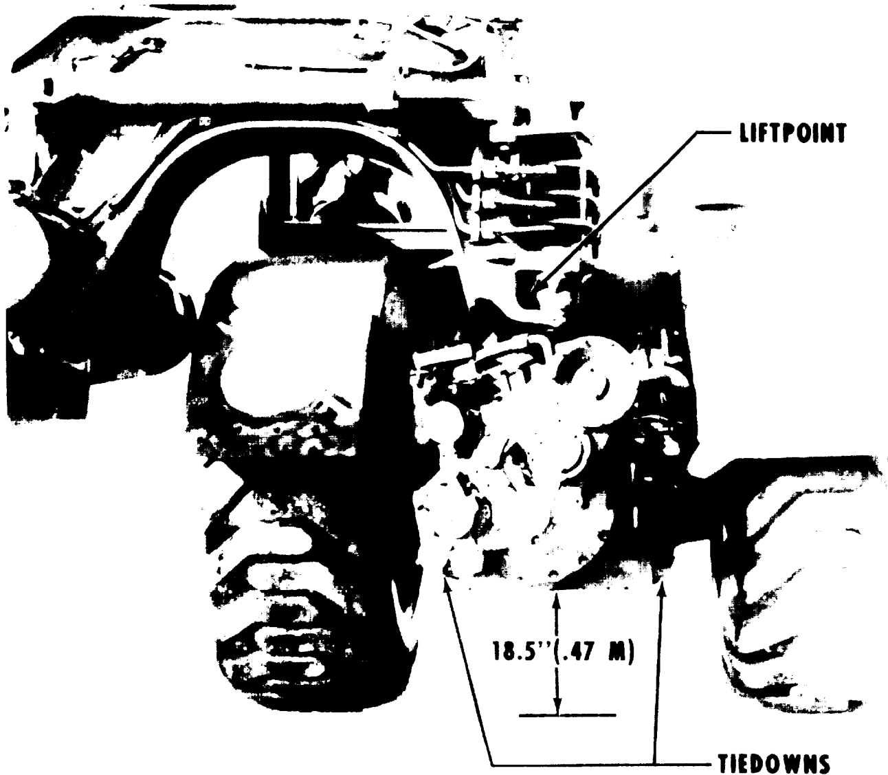
Figure 6-1. Tractor-Scraper front lift points and tiedown points
