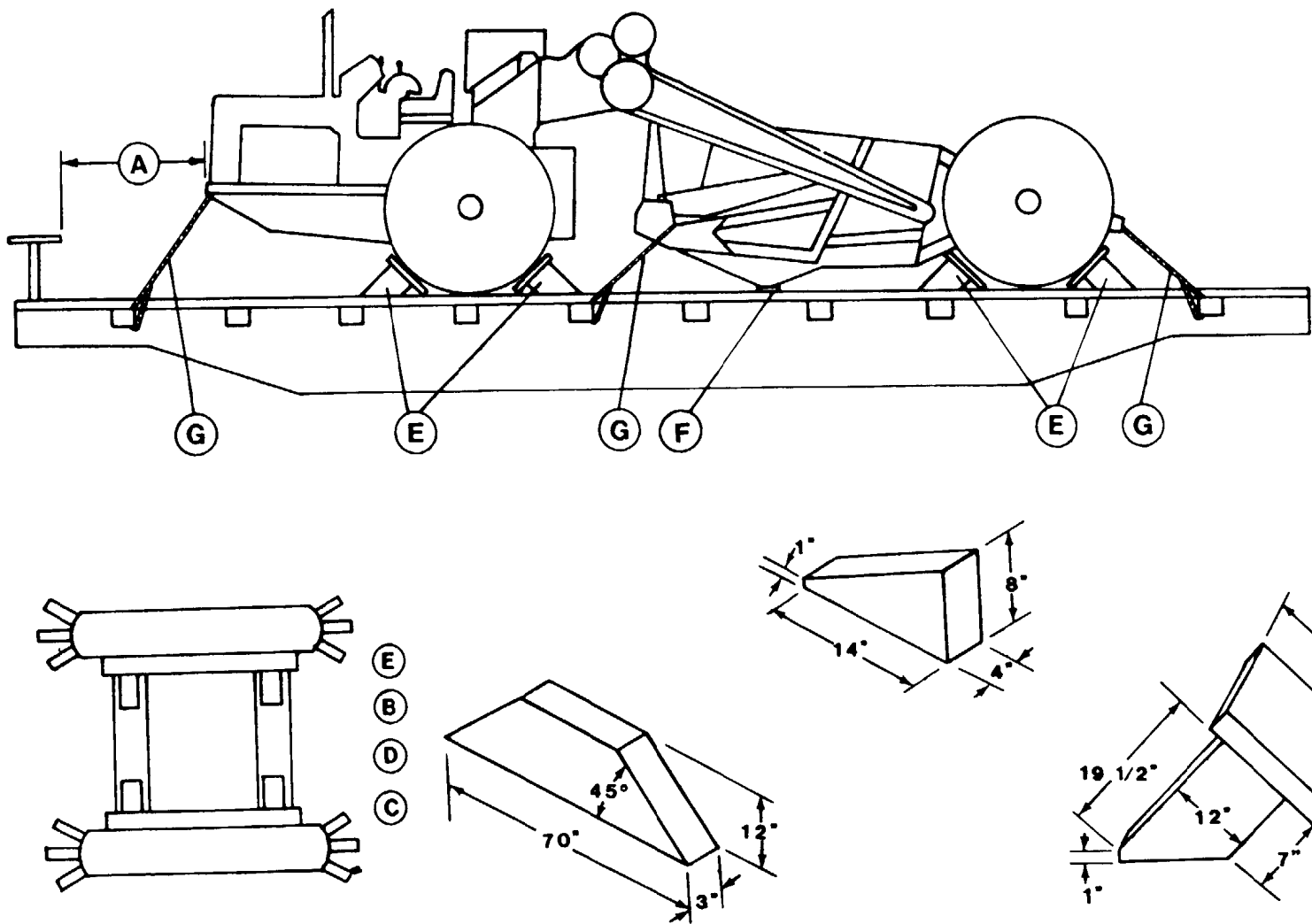
Figure 7-1. Side view of tractor-scraper loaded and restrained on a general-purpose flatcar.
