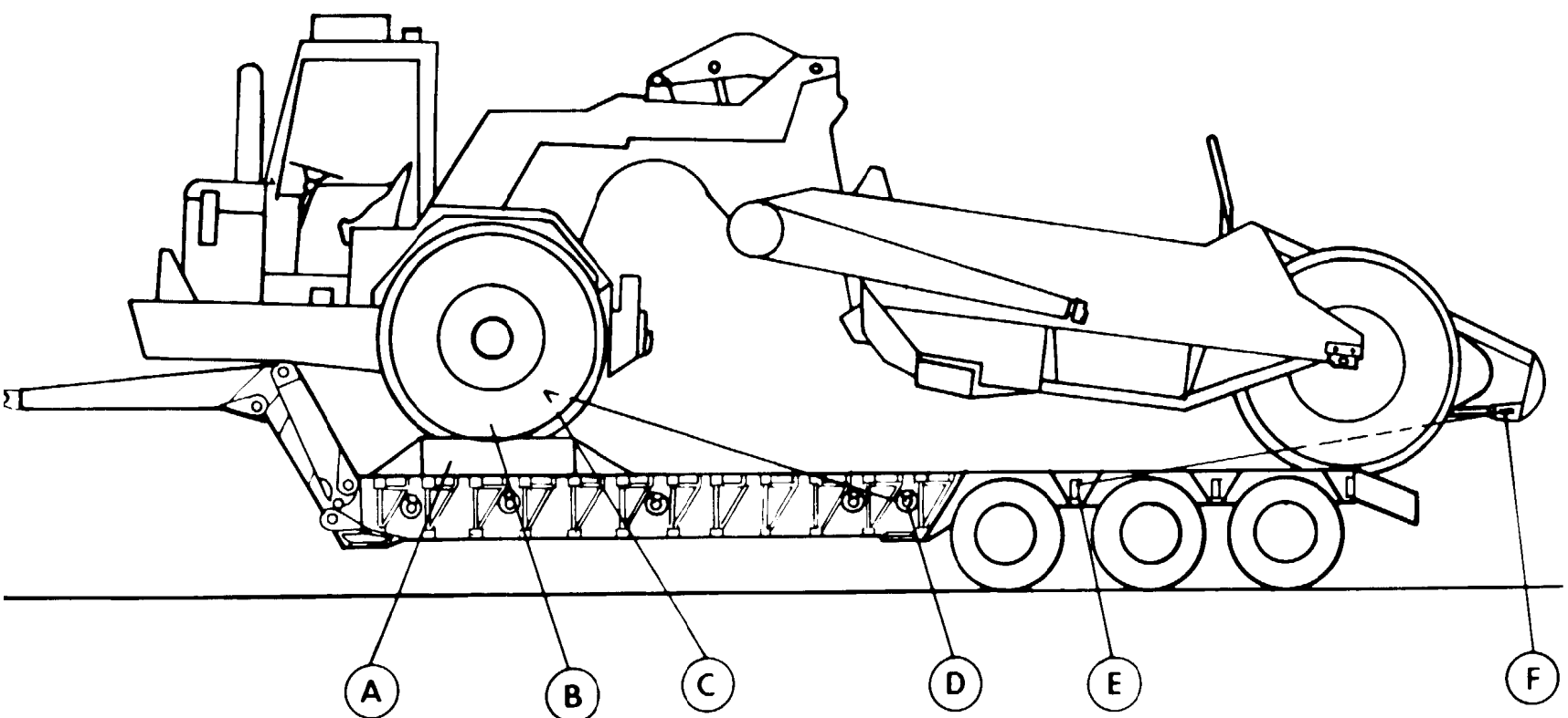
Figure 5-1. Tiedown diagram of the tractor-scraper on a semitrailer, M870.
