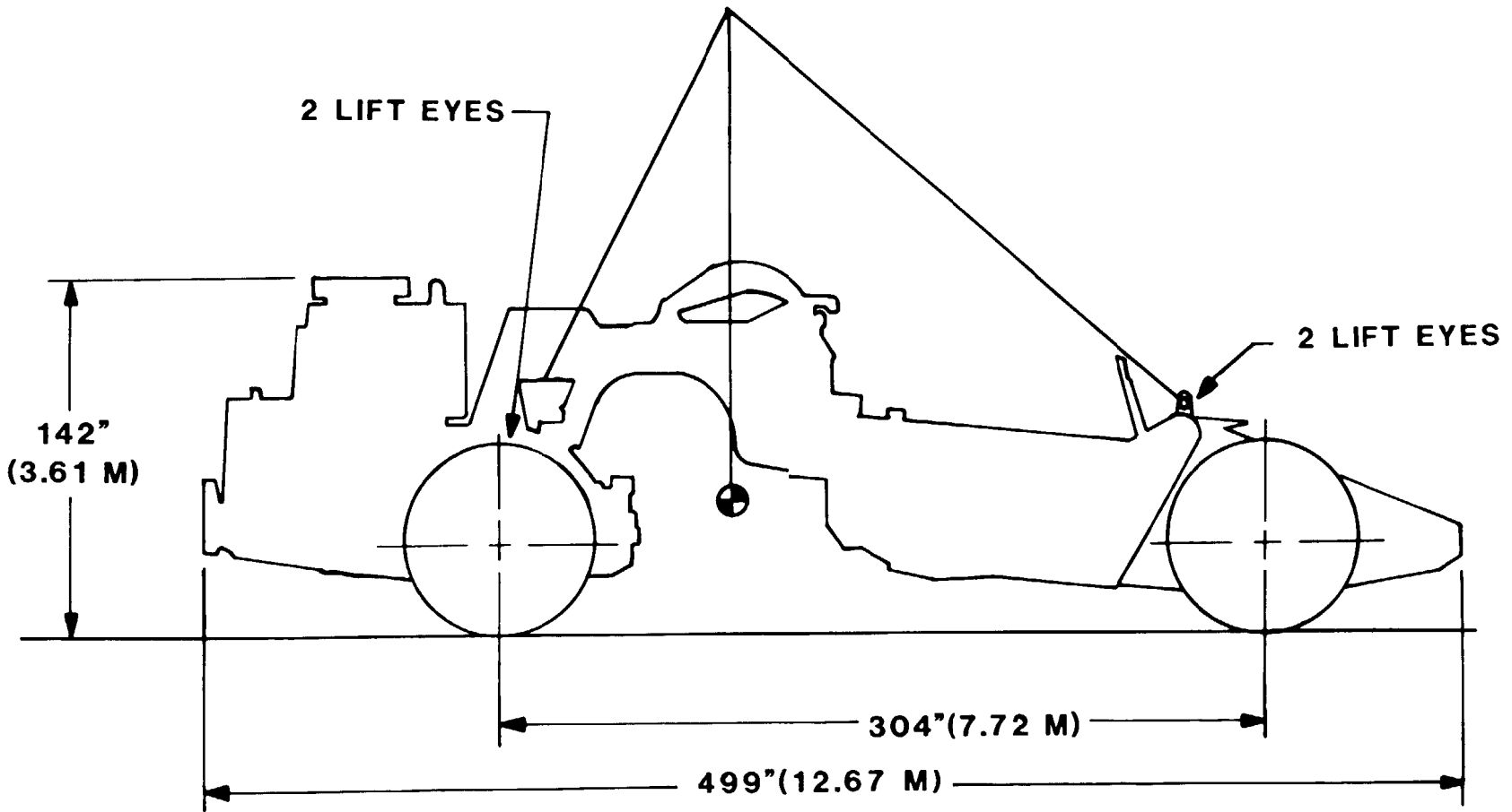
Figure 6-2. Lifting diagram for tractor-scraper.
