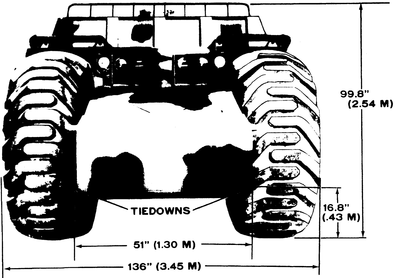
Figure 2-3. Rear view of tractor-scraper, wheeled M621B.
