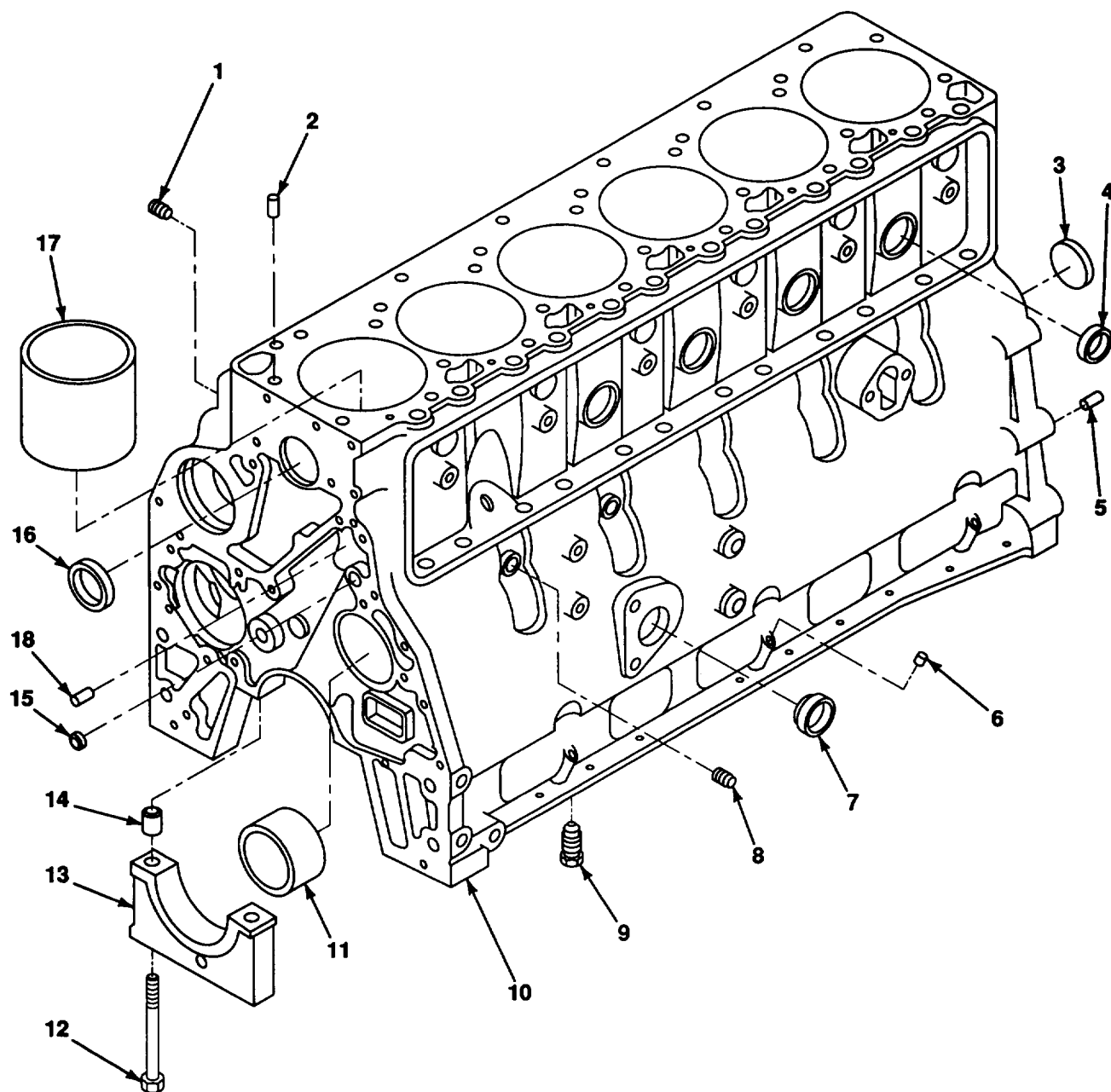
Figure 2. Cylinder Block
