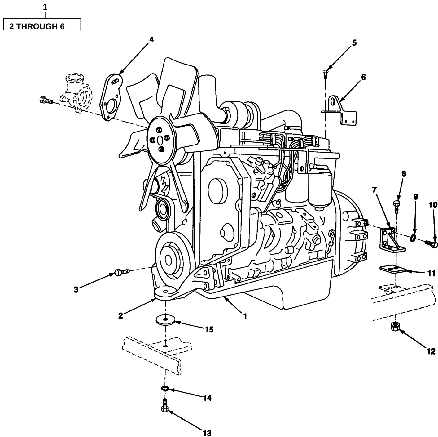
Figure 1. Drive Engine Assembly
