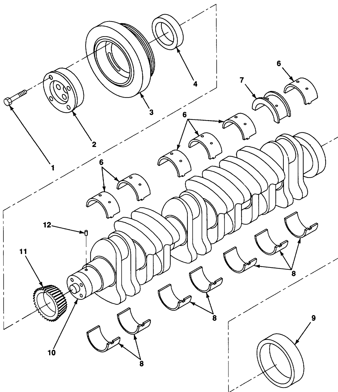
Figure 4. Crankshaft, Vibration Dampener
